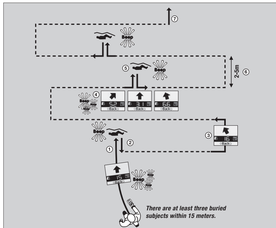
Search tactics with multiple burials in close proximity in analog mode
